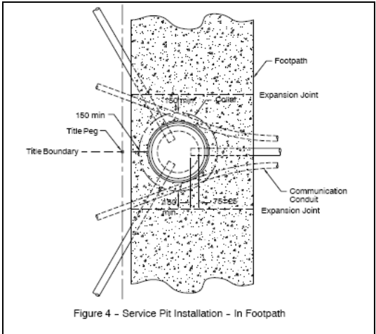
Compliant Installation of a Service Pit (minimum 150mm from any edge of the footpath including expansion joints) Extract from Technical Standard GS021
